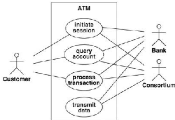
Figure 13.1 Use case diagram for the ATM. Use cases are in the box
