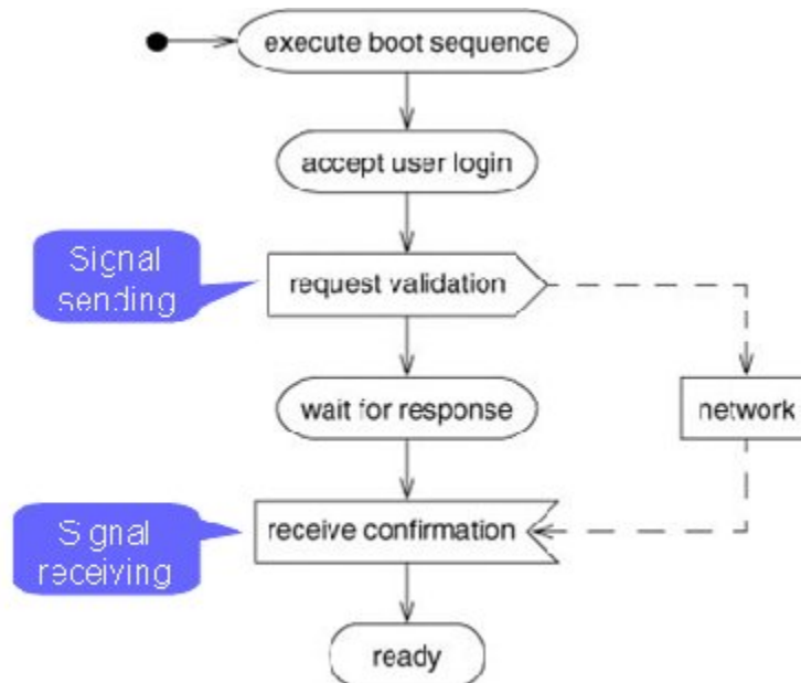
Figure 8.7 Activity diagram with signals. Activity diagrams can show line control via sending and receiving events.
